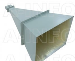
LB-650-20-C-NF Standard Gain Horn Antenna 1.12-1.7GHz 20dB Gain N Type Female
