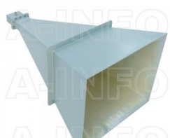
LB-650-20-C-7/16F Standard Gain Horn Antenna 1.12-1.7GHz 20dB Gain 7/16(DIN) Female
